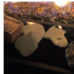
Shale
